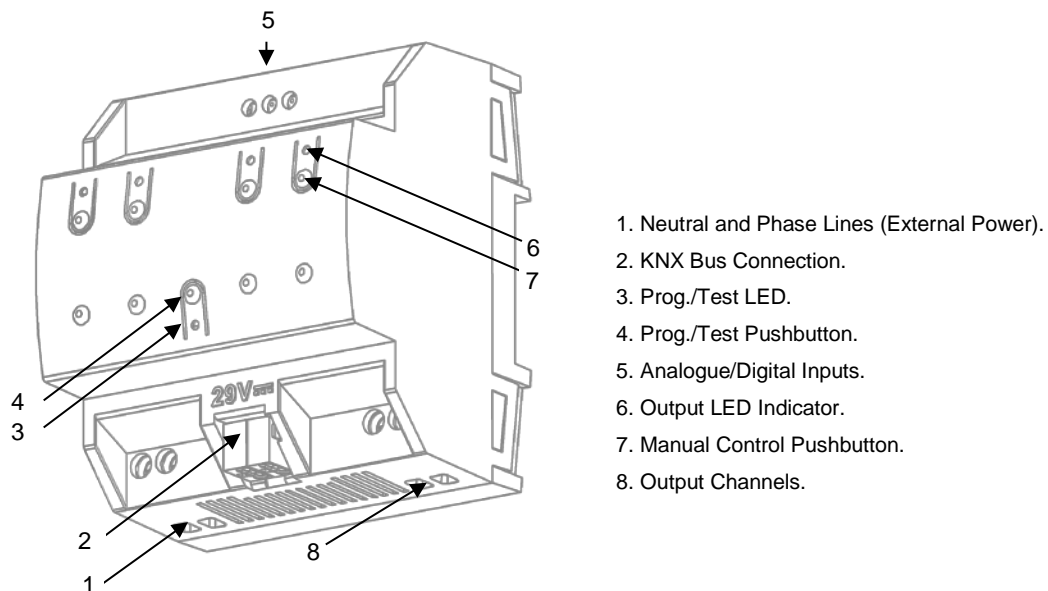
Figure 3 DIMinBOX DX2 - Element Diagram.
