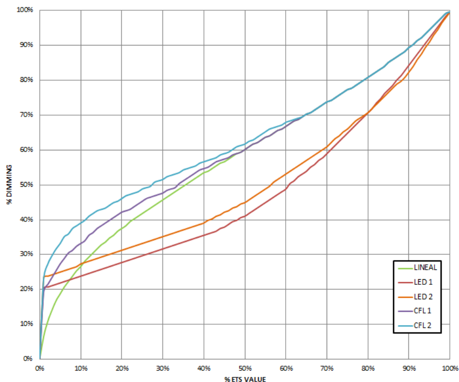
Figure 6 Dimming Patterns for LED and CFL loads.
