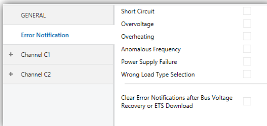
Figure 20 Error Notification.
